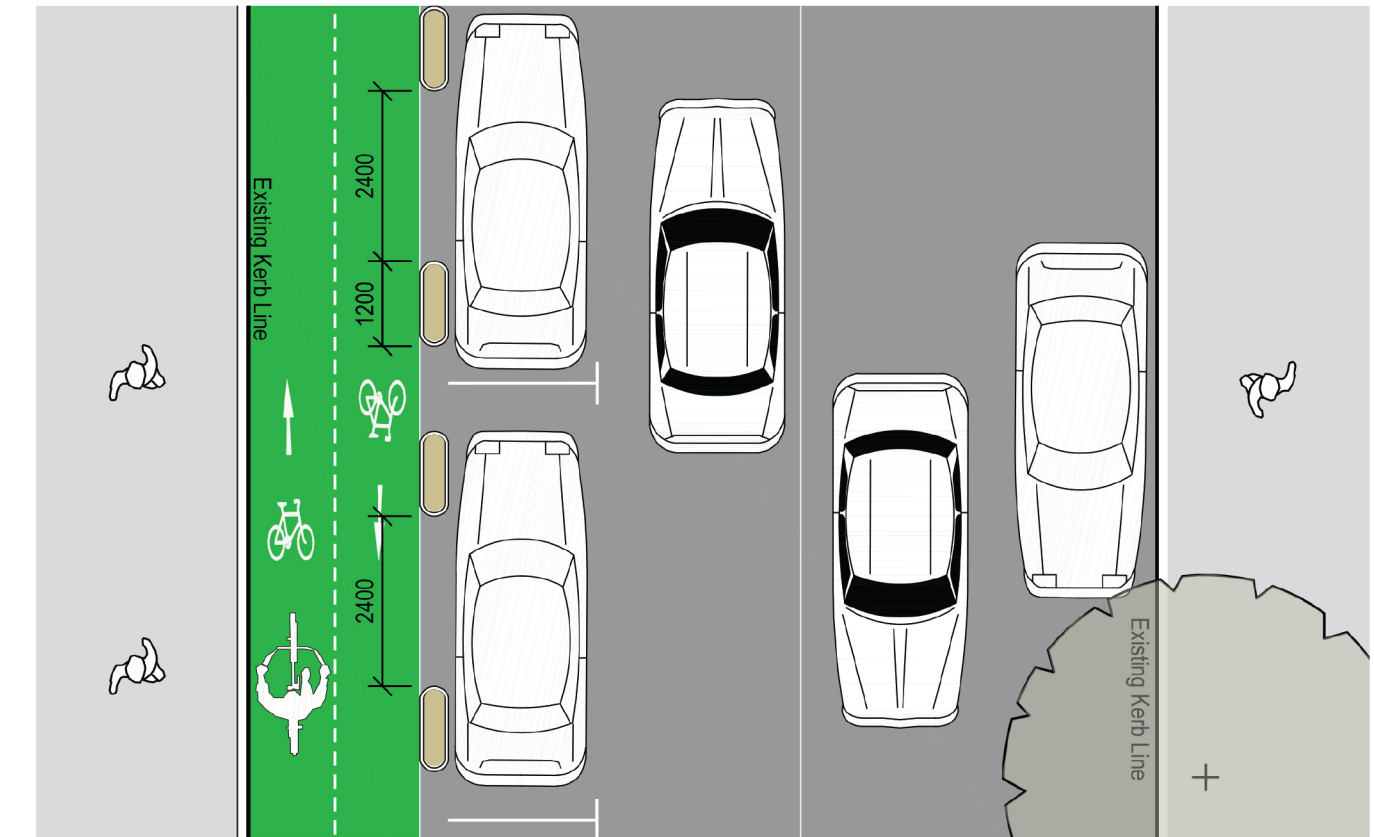
TYPICAL INTERRUPTED MEDIAN SEPARATED CYCLEWAY
