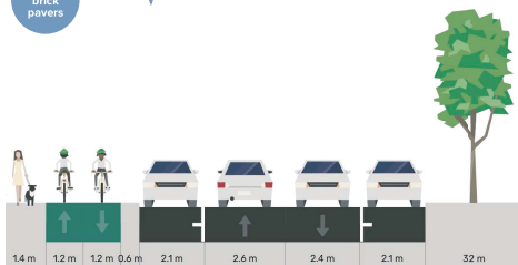
TYPICAL CROSS-SECTION D-D
