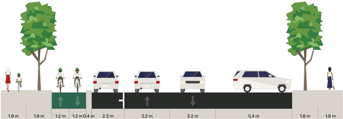
TYPICAL CROSS-SECTION B-B
