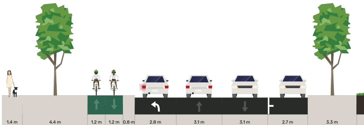
TYPICAL CROSS-SECTION C-C
