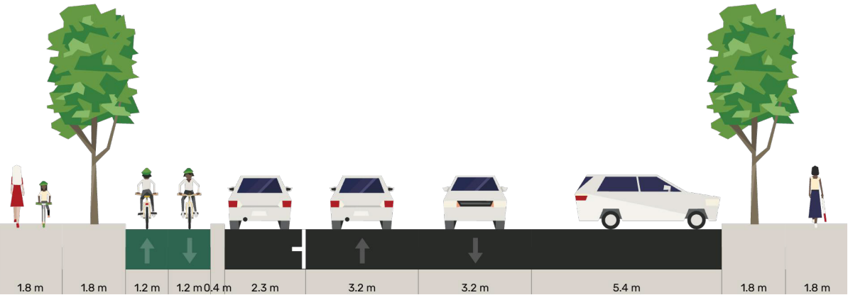
TYPICAL CROSS-SECTION A-A
