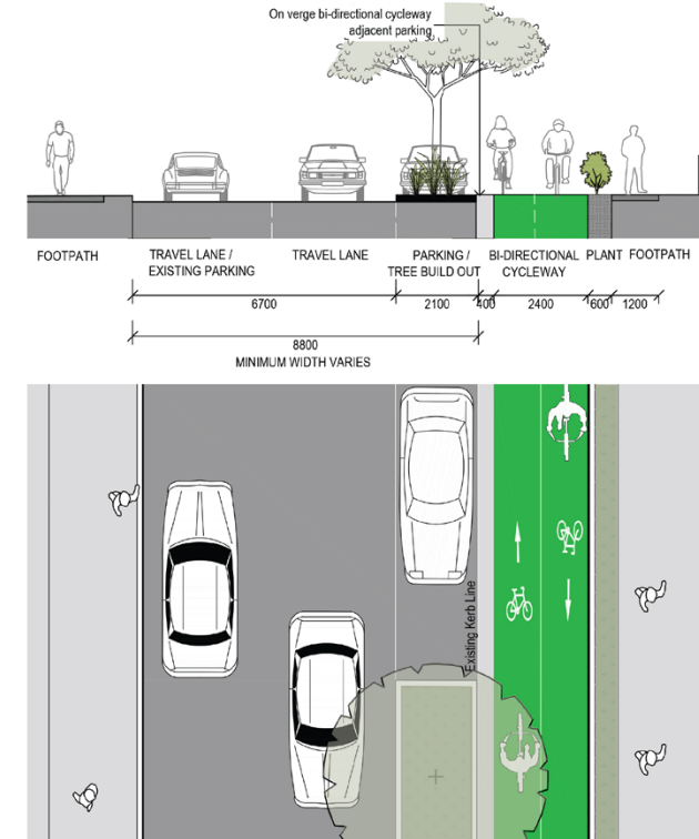
TYPICAL ON VERGE CYCLEWAY WITH IN ROAD PLANTING
