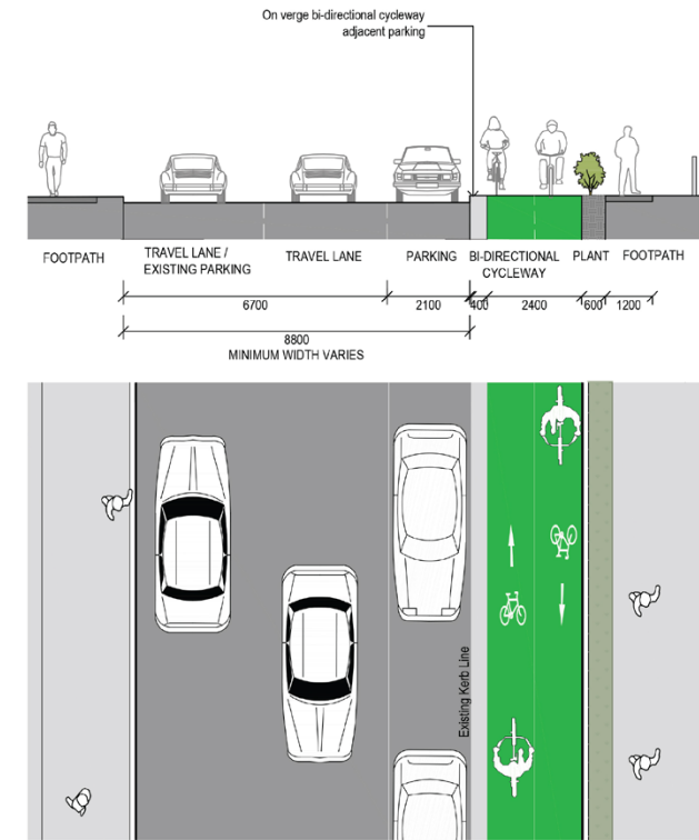
TYPICAL ON VERGE CYCLEWAY
